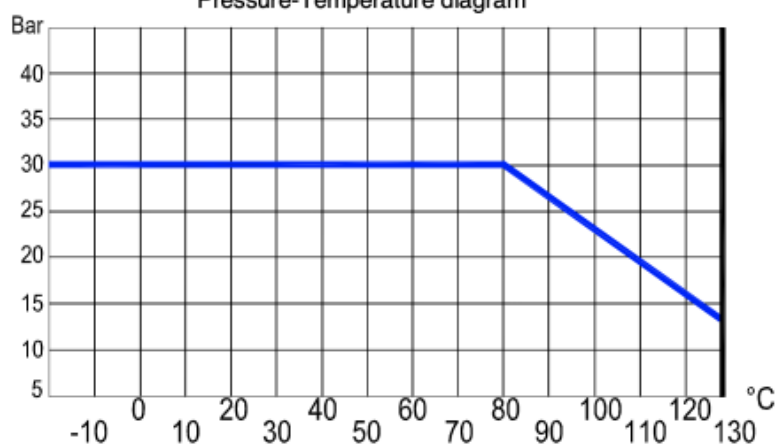
Diagramma Pressione-Temperatura Pressure-Temperature diagram
